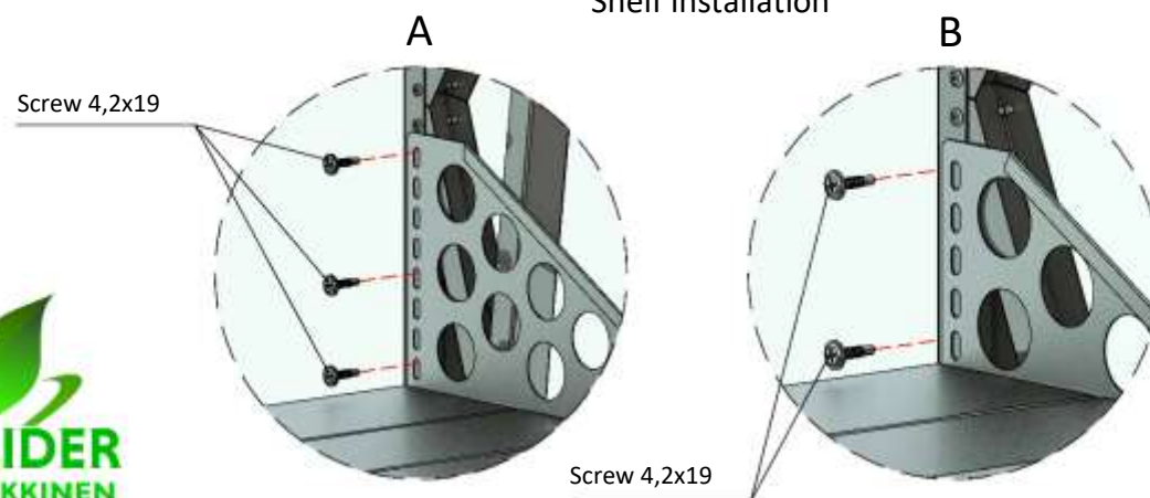
Shelf installation
