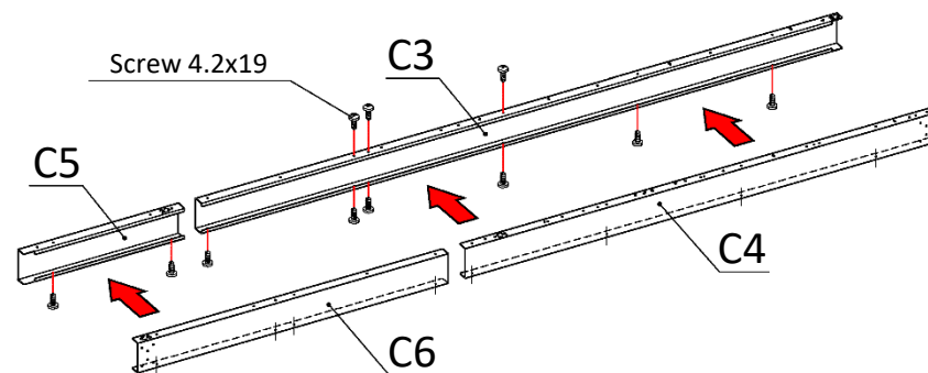
End beam C3+C4+C5+C6
