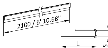
H- profile (1500 mm)
