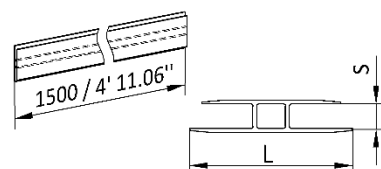
H- profile (2380 mm)
