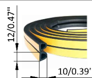
Rubber profile
